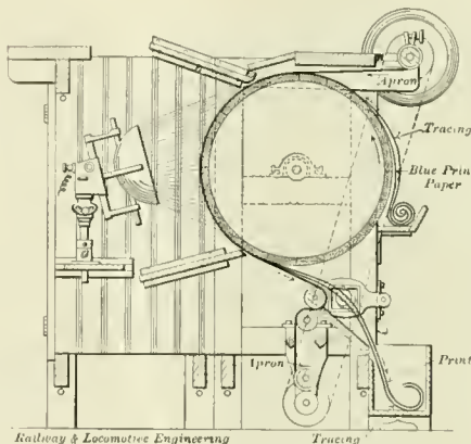
BLUE PRINT APPARATUS.
